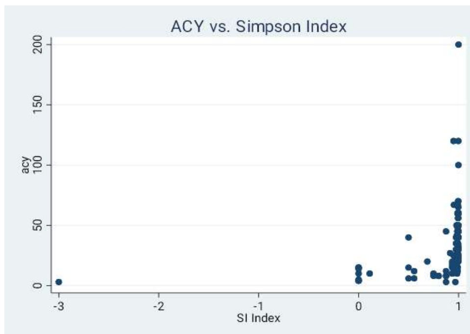
Figure: Relationship between Average crop yield and Simpson index
